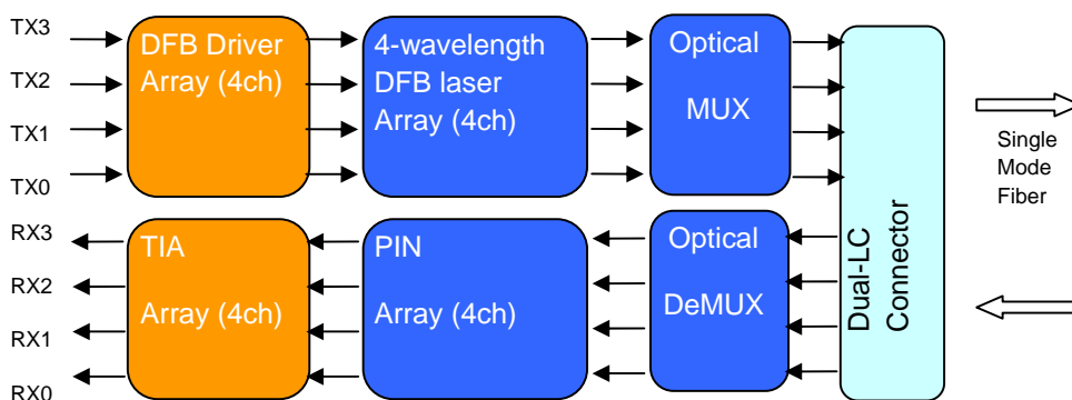
Figure 1: 40Gb/s QSFP GR4 Transceiver Block Diagram
