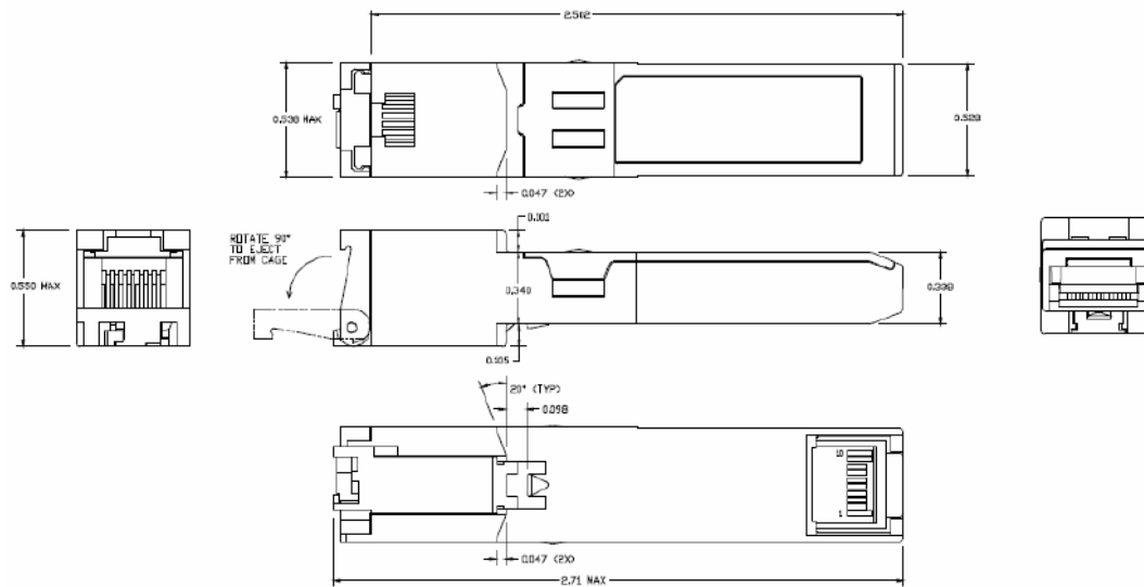
Figure 2. Mechanical dimensions
